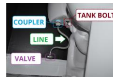
Toilet plumbing
